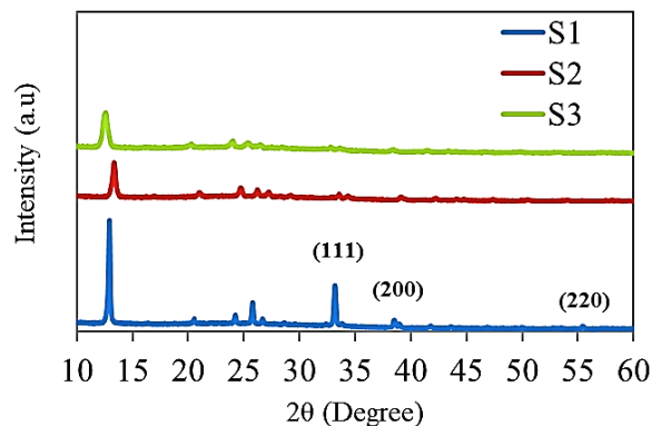
Fig. 1. XRD patterns for the as-deposited samples. S1, S2 and S3 resemble pure, 0.46 at%, and 1.51 at%, respectively
